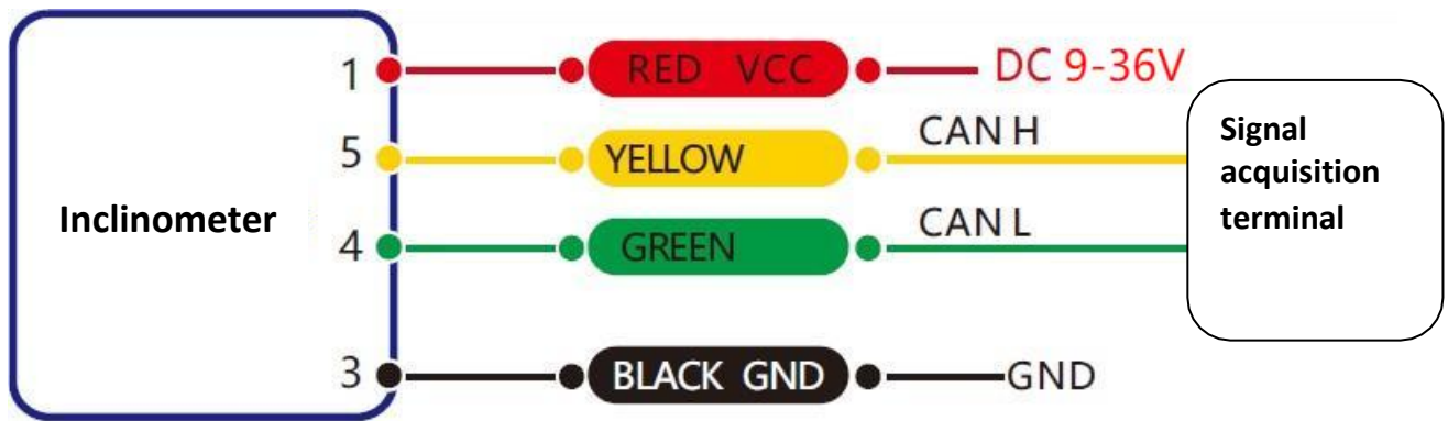
CAN总线接线图 CAN Bus Wiring Diagram
