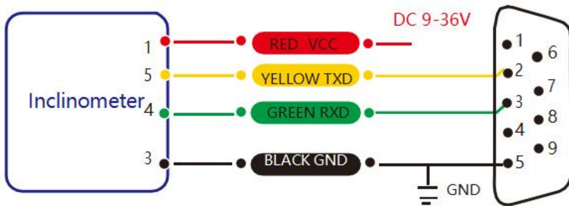
RS 232 wiring diagram
