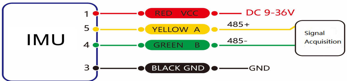
RS 485 connection diagram
