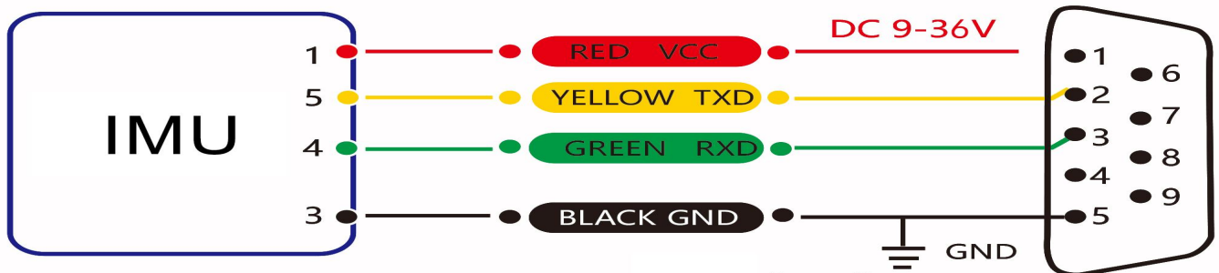
RS 232 connection diagram
