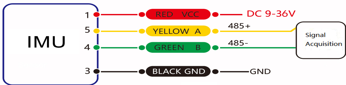
RS 485 connection diagram
