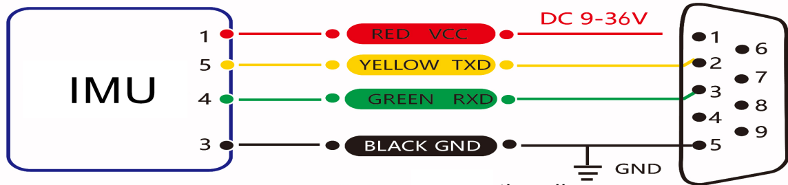
RS 232 connection diagram
